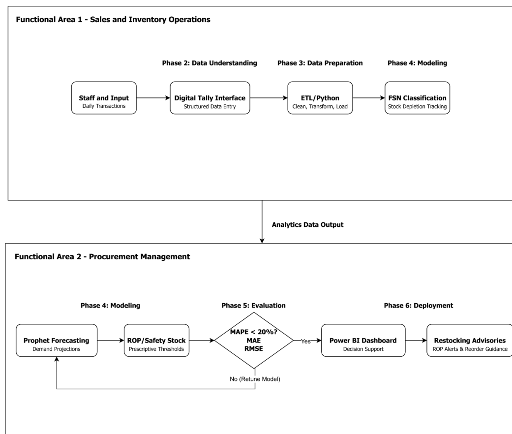
Figure 1. Conceptual Framework of Data Integration
