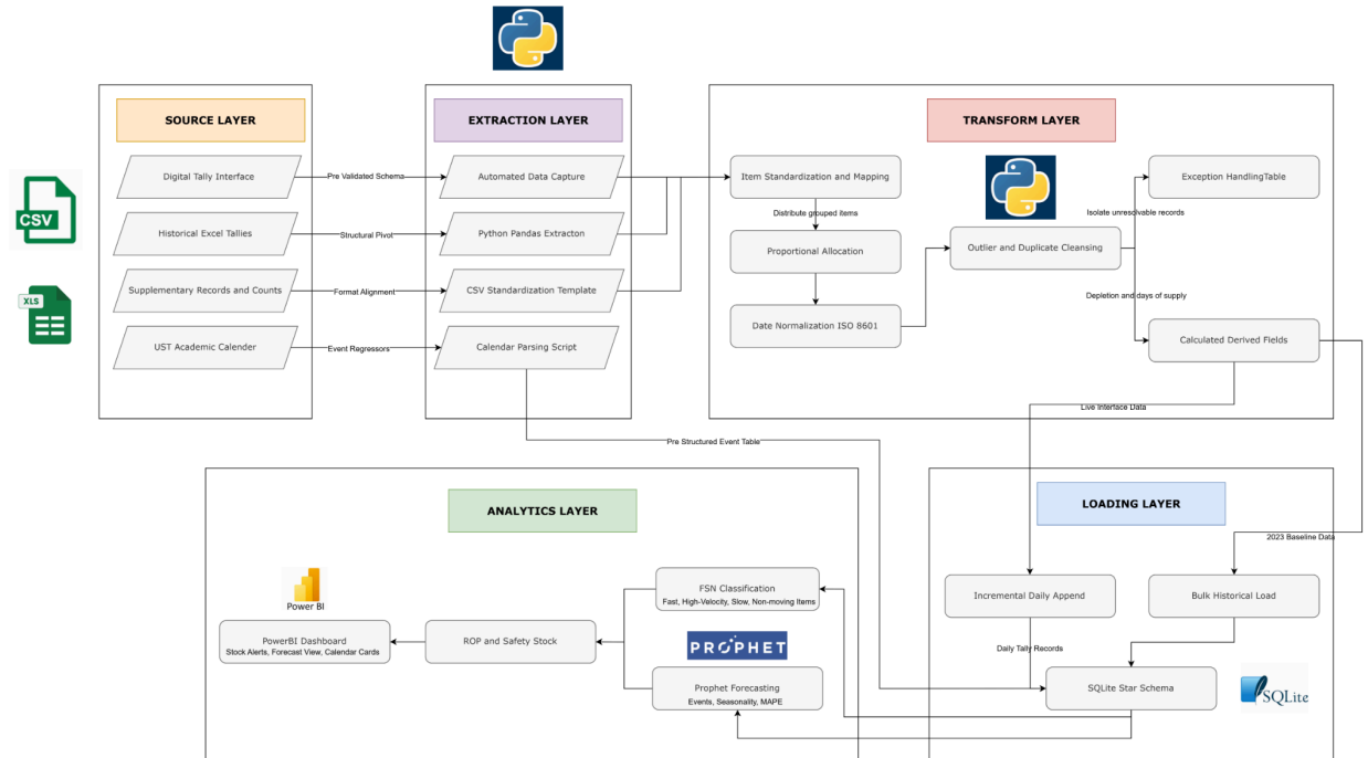
Figure 4. Data Pipeline for the USTore Demand Forecasting and Prescriptive Inventory Management Dashboard
